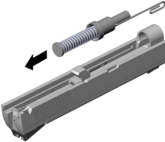
Figure 6: Recoil Spring Assembly Removal
