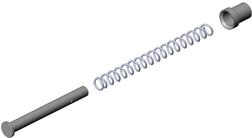
Figure 7: Recoil Spring Assembly Separation
